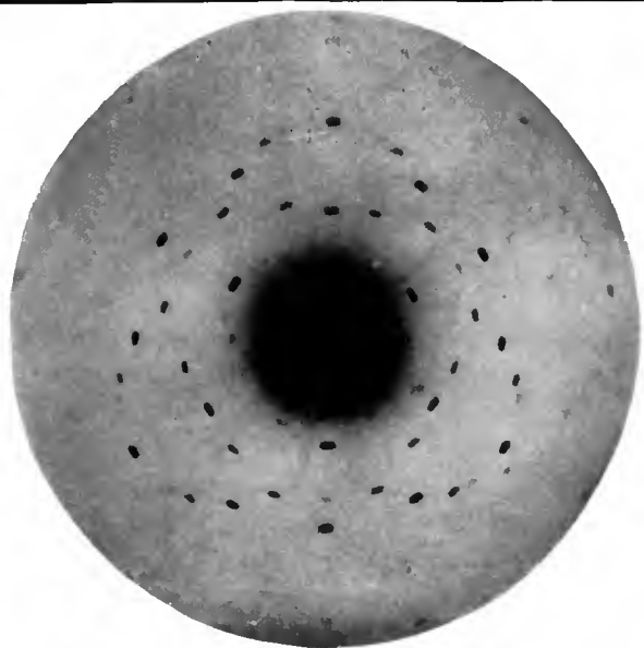
FIG. 5.—Laue X-ray Photograph Through the Basal Plane of Penninite.
