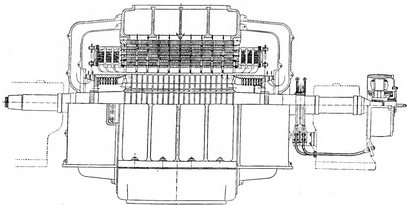
FIG. 1.—Longitudinal Section of Large 2-Pole Turbo-Alternator (Metropolitan-Vickers Electrical Co., Ltd.).
