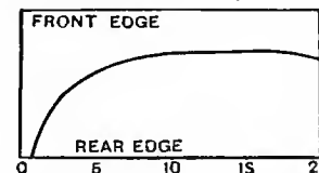
FIG. 6c.—Travel of Centre of Pressure as Angle of Attack varies.
