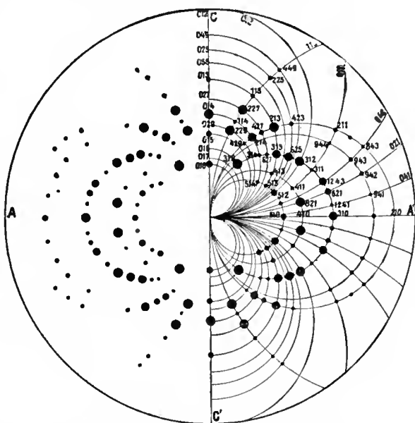
FIG. 8.—Stereogram of Laue Photograph of Anhydrite on the Face (010).
