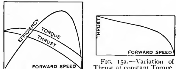
FIG. 15.—Variation of Thrust, Torque and Efficiency of an Airscrew with forward speed at constant rate of revolution.
