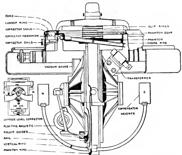
FIG. 3.—Starboard view of frame. West view of compass.
