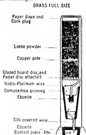
FIG. 2.—Tube, Vent Sealing, Electric W. P.
