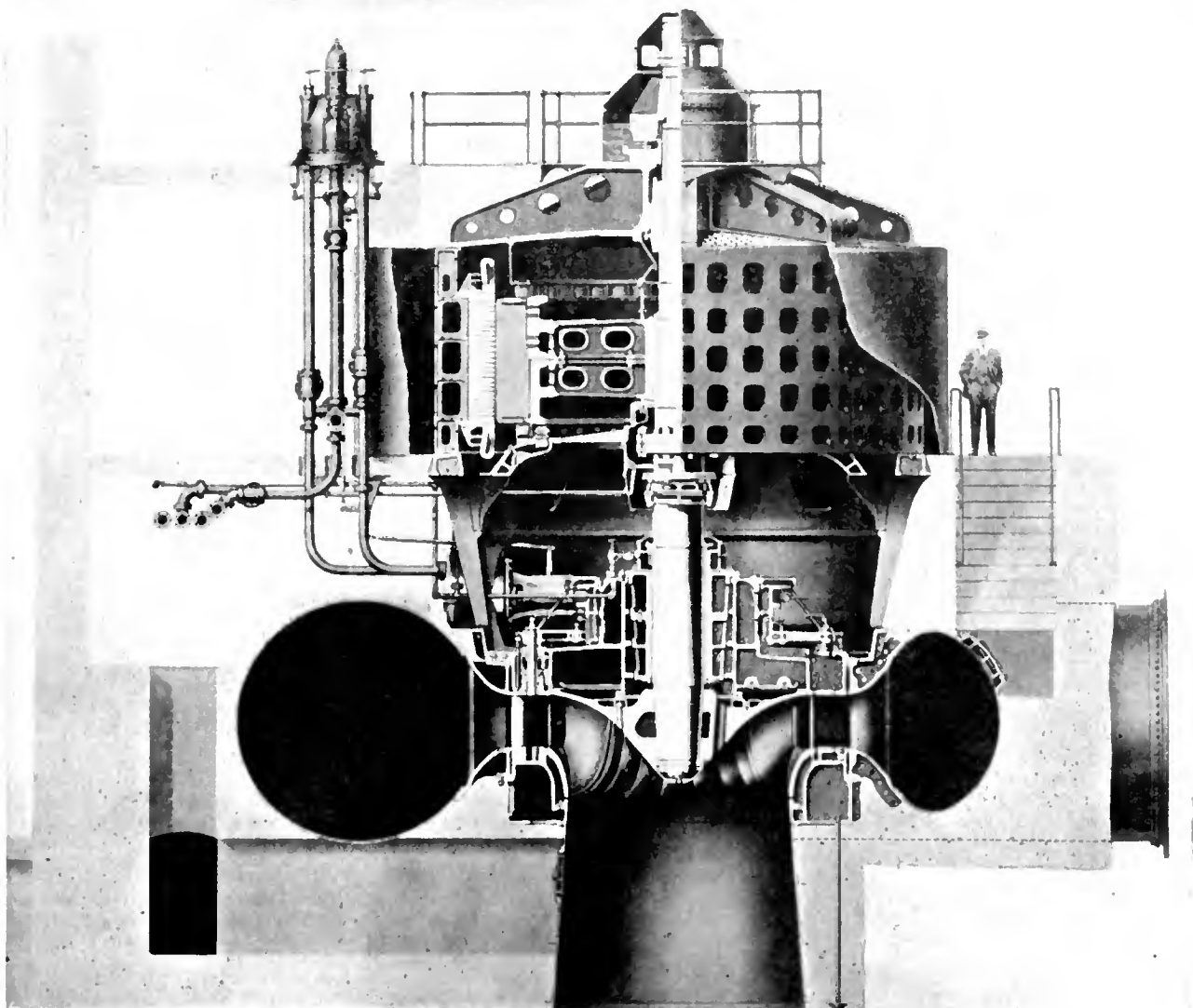
FIG. 3.—32,500-kva. Combined Water-Turbine and Alternator.
