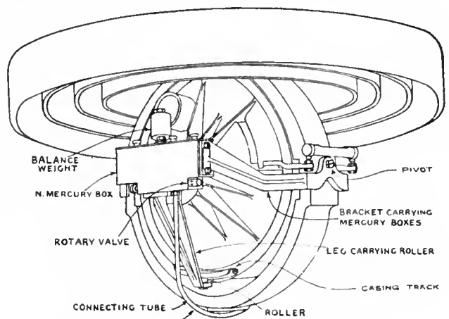
FIG. 4.—General view of mercury control.
