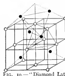
FIG. 10.—“Diamond Lattice” representing diamond when the atoms are all of the same kind, or zinc-blende when of two kinds.
