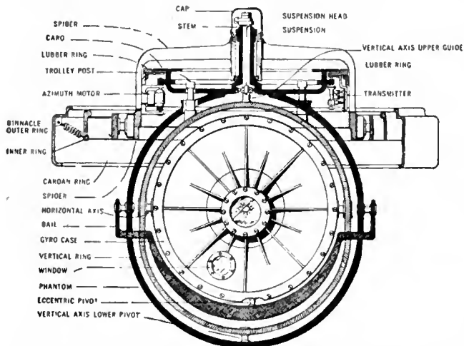
FIG. 1.—Thwartship section of frame. South view of compass.
