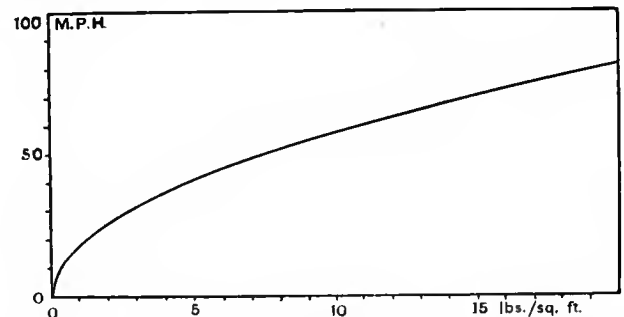
FIG. 10.—Curve showing lowest speed of flight possible with given wing-loading and the usual thin wings.
