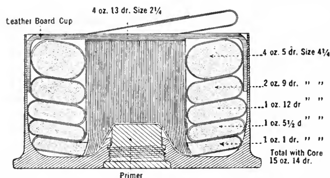
FIG. 1.—4-5 in. Q. F. Howitzer Cartridge.
