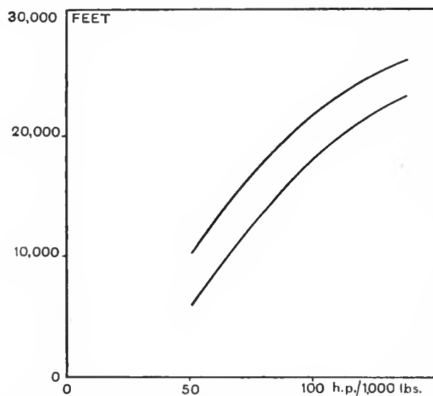
FIG. 12.—Diagram showing greatest effective height attainable by British military aeroplanes. These vary between the upper and lower curves. The base is engine power at ground level per 1,000 pounds of total weight.
