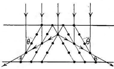
FIG. 7.—Reflection of X Rays by Planes of Particles; production of spots in the Laue photographs.
