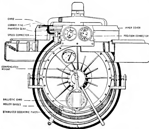
FIG. 2.—Aft view of frame. North view of compass.
