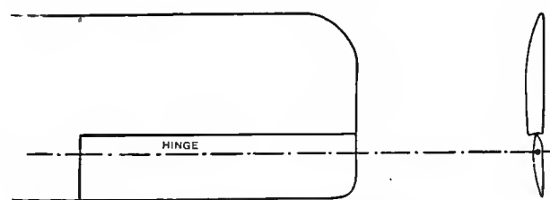
EXAMPLE OF SET-BACK HINGE BALANCE
