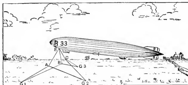
G1, G2, G3. Denotes swivelling Pulley attached to Ground Bollards S Denotes Mooring Point, A, B, C. Denotes Rings.
