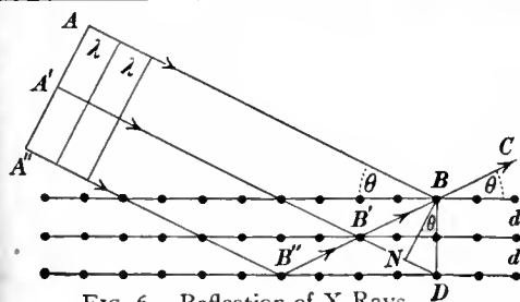
FIG. 6.—Reflection of X Rays by Planes of Particles.
